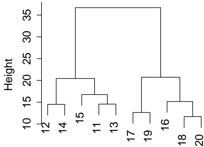
hierarchical clustering
